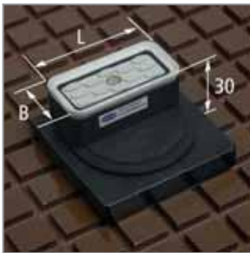
Suction cup ISMUP Cup 2 80x40x30 (shown here with Mono-Base)
